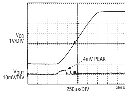
Power-On Reset Glitch to Zero Scale
